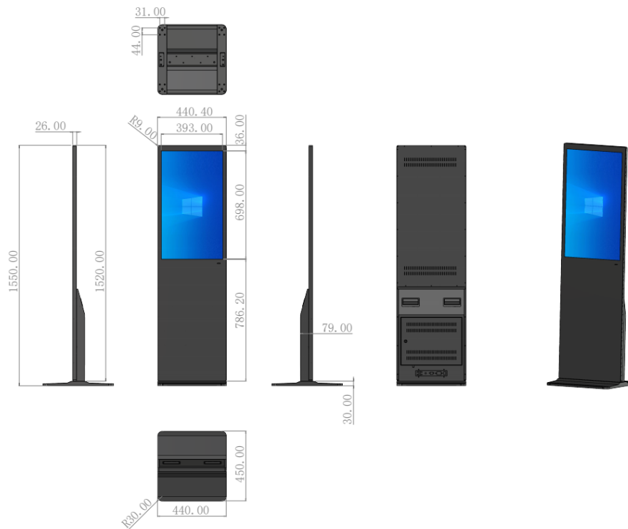
LF-FSA-32 Dimensions (mm)
