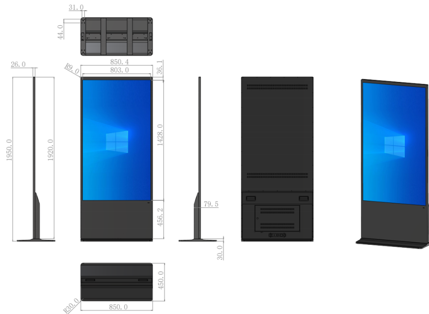
LF-FSA-65 Dimensions (mm)
