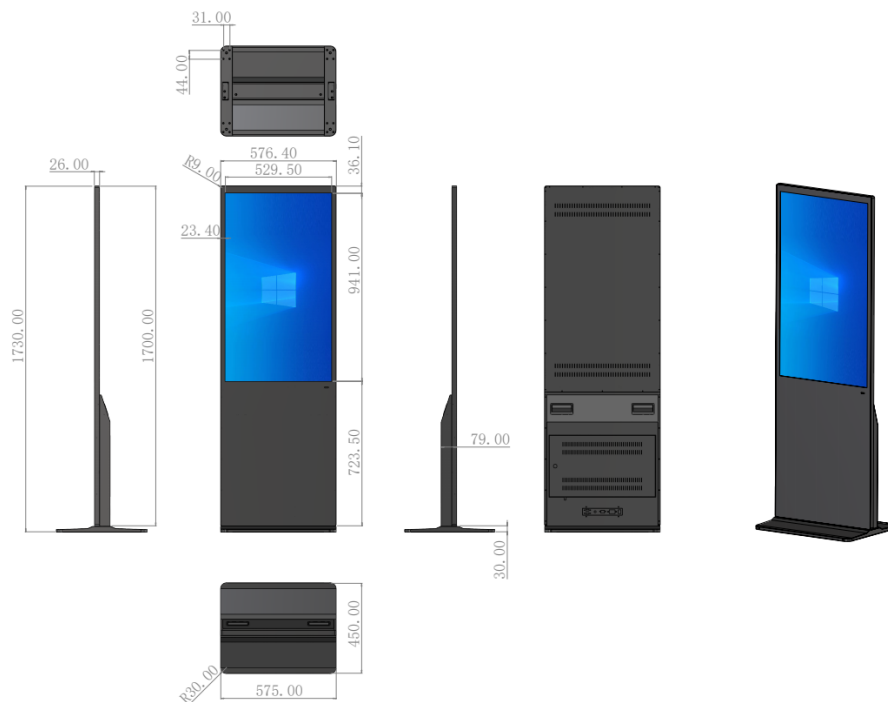
LF-FSA-43 Dimensions (mm)
