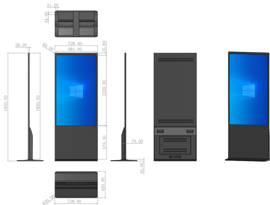
LF-FSA-55 Dimensions (mm)
