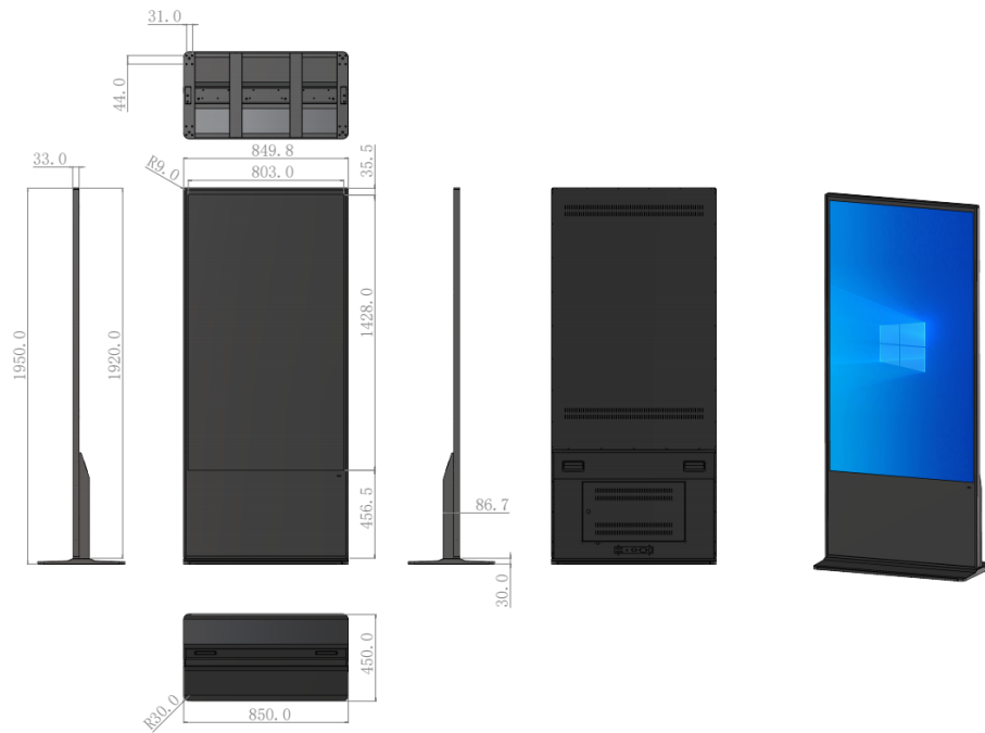
LF-FST-IR-65 Dimensions (mm)
