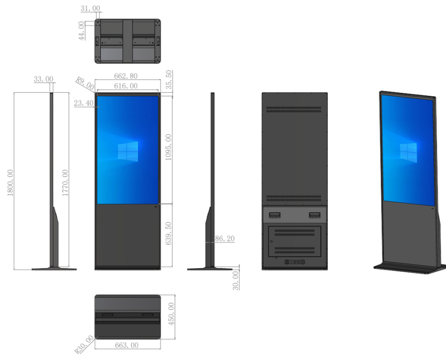
LF-FST-IR-50 Dimensions (mm)
