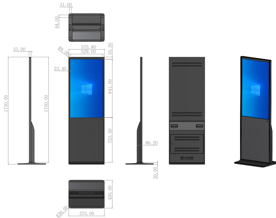
LF-FST-IR-43 Dimensions (mm)
