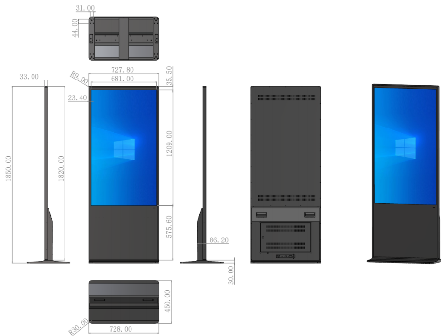
LF-FST-IR-55 Dimensions (mm)
