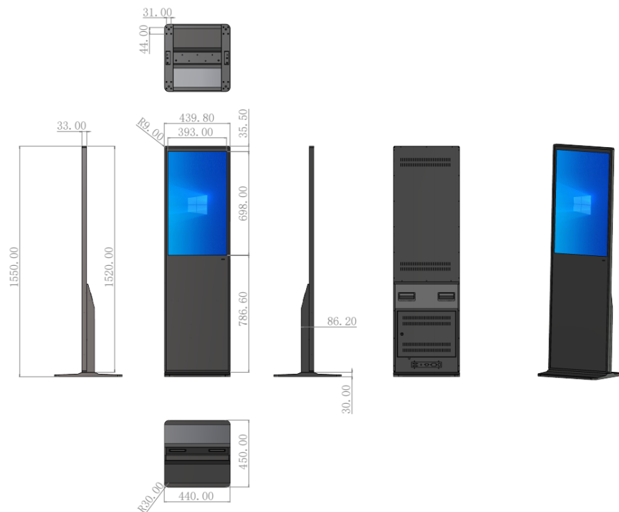
LF-FST-IR-32 Dimensions (mm)
