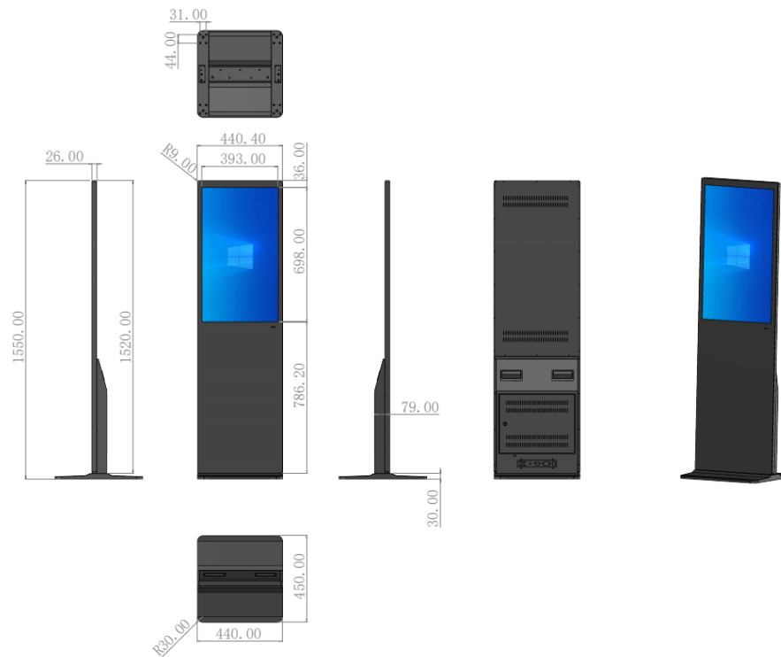
LF-FST-PC-32 Dimensions (mm)
