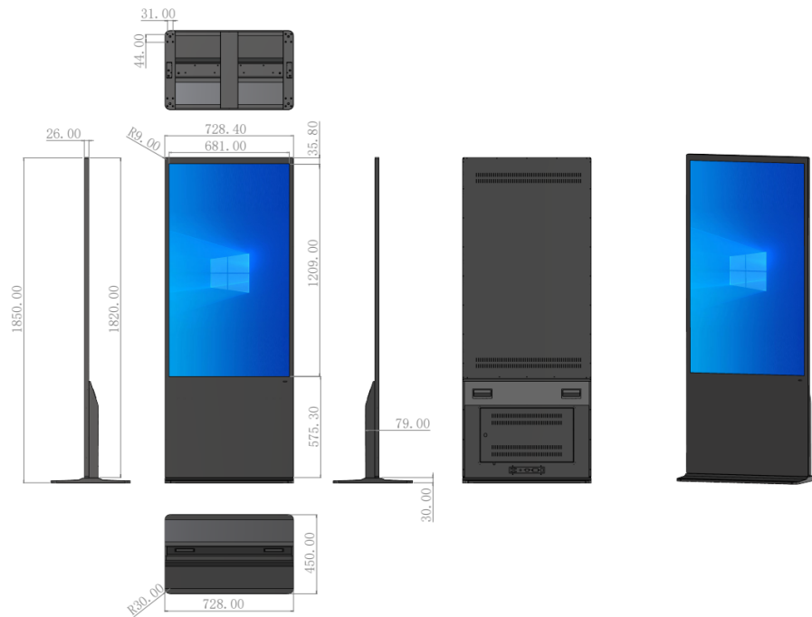
LF-FST-PC-55 Dimensions (mm)
