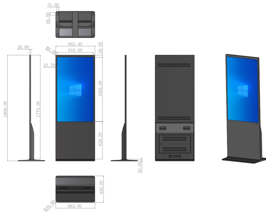
LF-FST-PC-50 Dimensions (mm)
