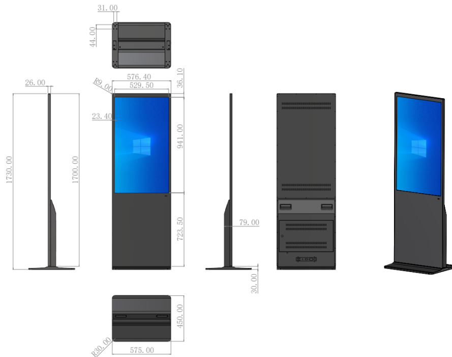
LF-FST-PC-43 Dimensions (mm)
