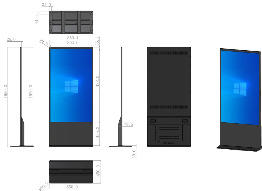
LF-FST-PC-65 Dimensions (mm)
