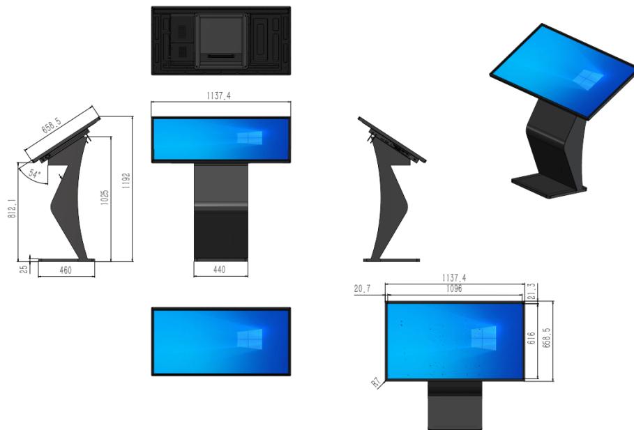
LF-HZK-IR-50 Dimensions (mm)
