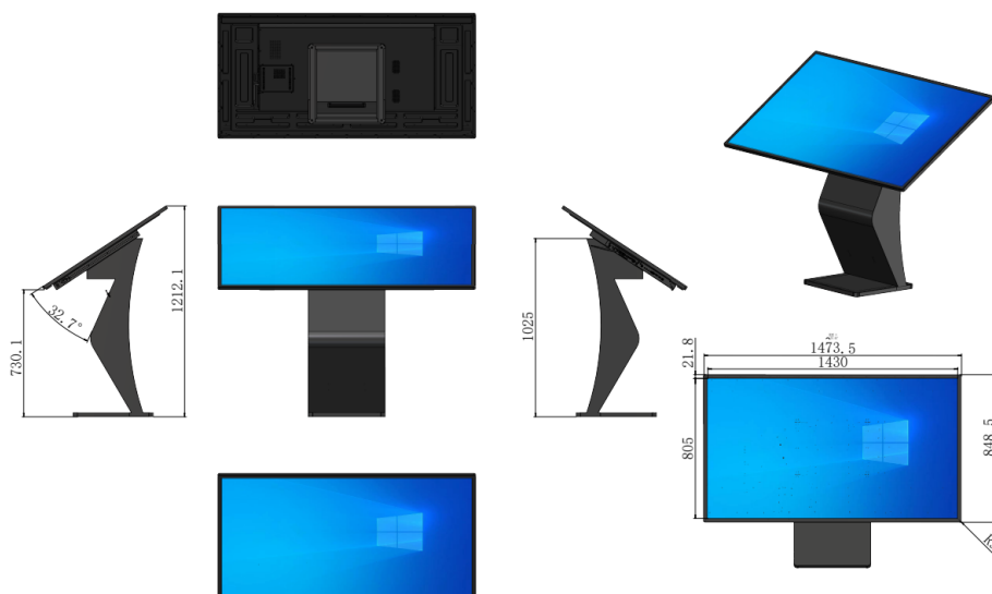
LF-HZK-PC-65 Dimensions (mm)
