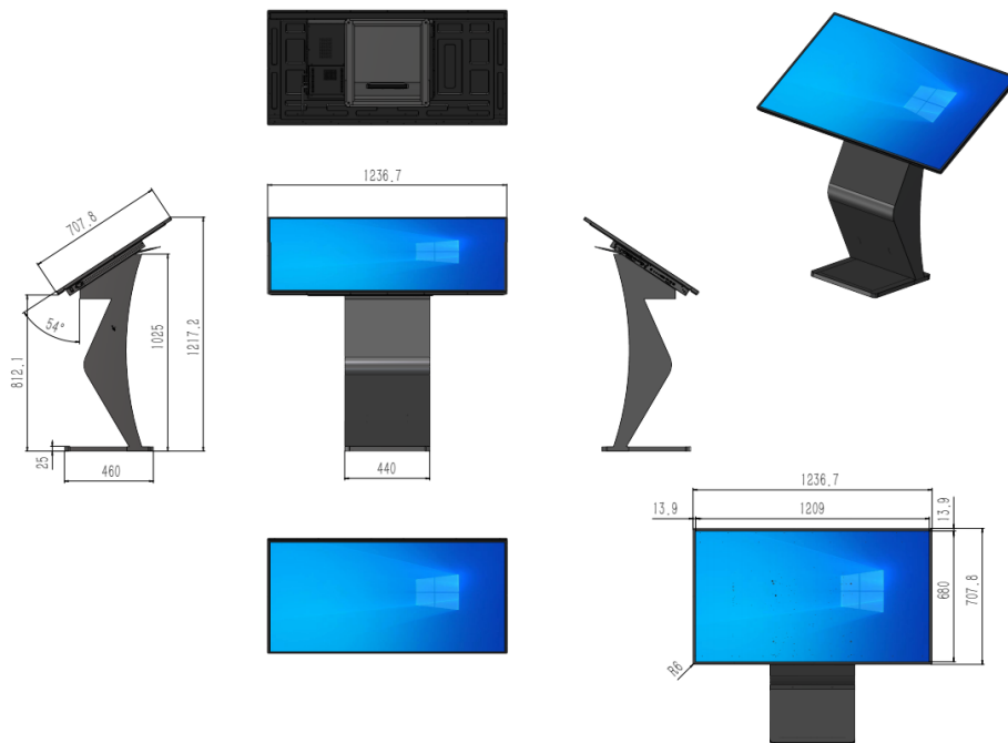
LF-HZK-PC-55 Dimensions (mm)
