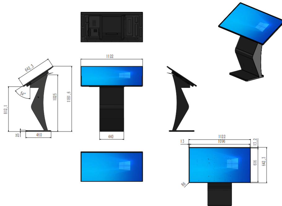
LF-HZK-PC-50 Dimensions (mm)
