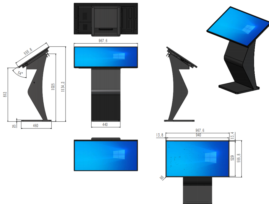
LF-HZK-PC-43 Dimensions (mm)
