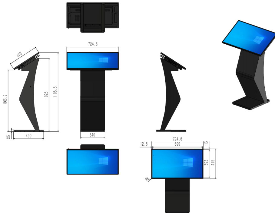
LF-HZK-PC-32 Dimensions (mm)
