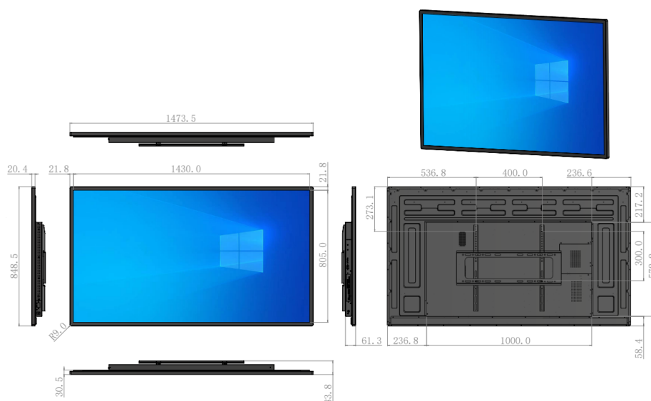
LF-WMT-PC-65 Dimensions (mm)
