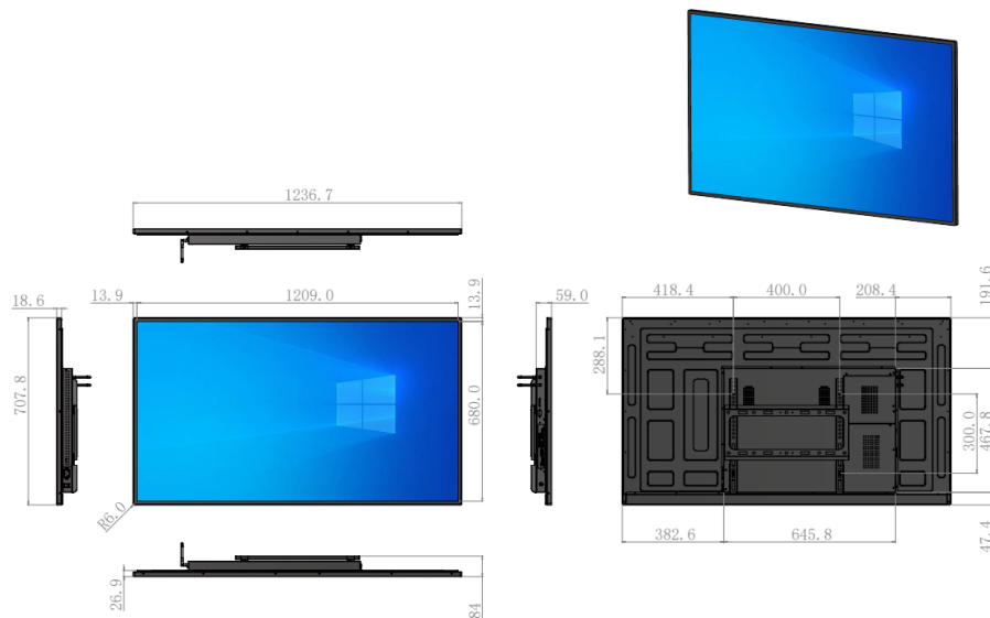
LF-WMT-PC-55 Dimensions (mm)
