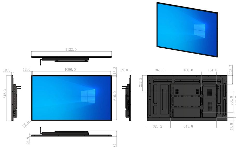
LF-WMT-PC-50 Dimensions (mm)
