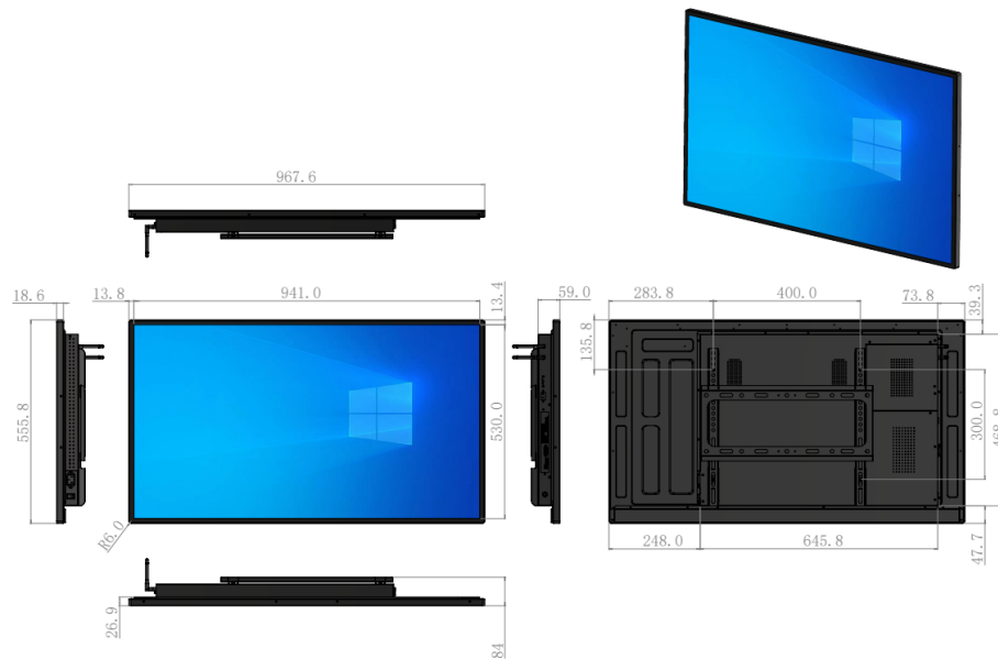
LF-WMT-PC-43 Dimensions (mm)
