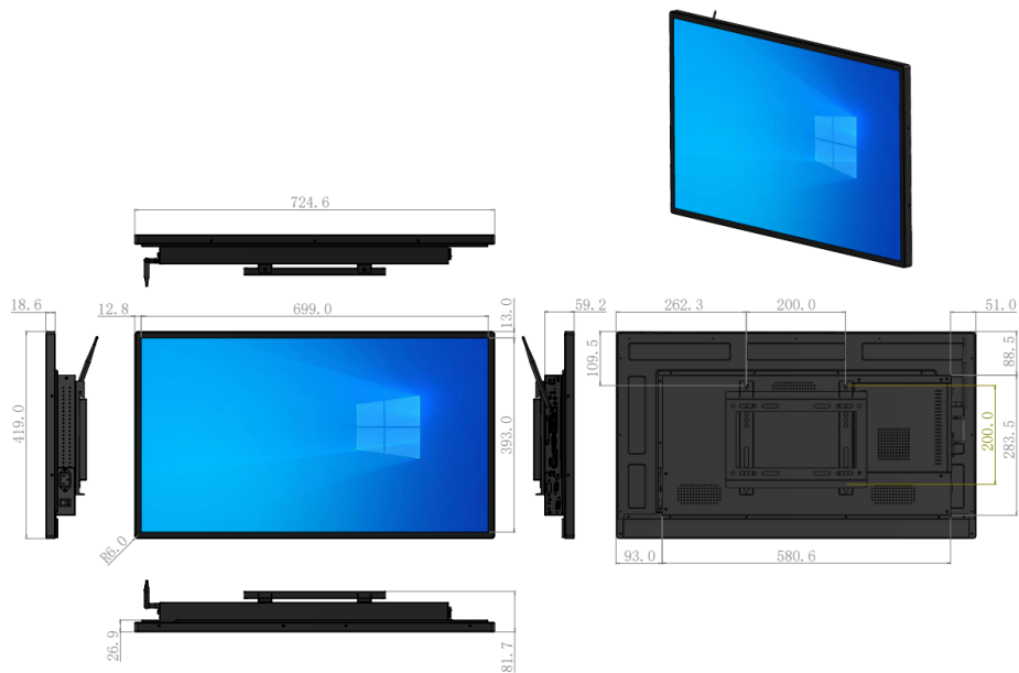
LF-WMT-PC-32 Dimensions (mm)
