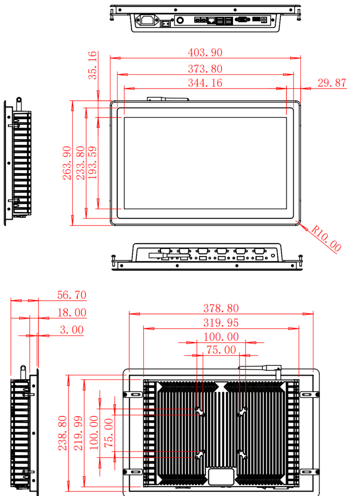
Dimension Drawings (Unit: mm)
