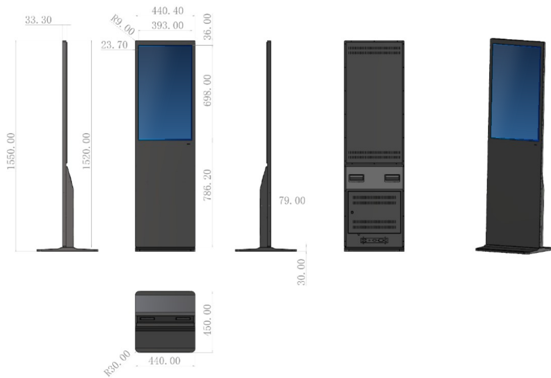
Dimensions (Unit: mm)
