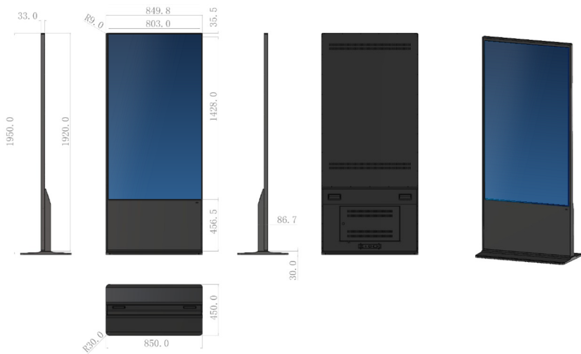
Dimensions (Unit: mm)
